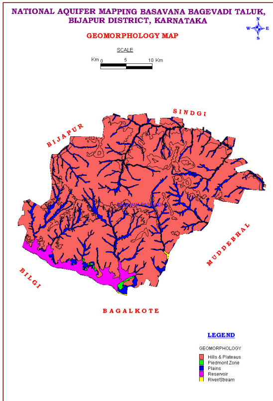
Figure 3: Geomorphology Map
